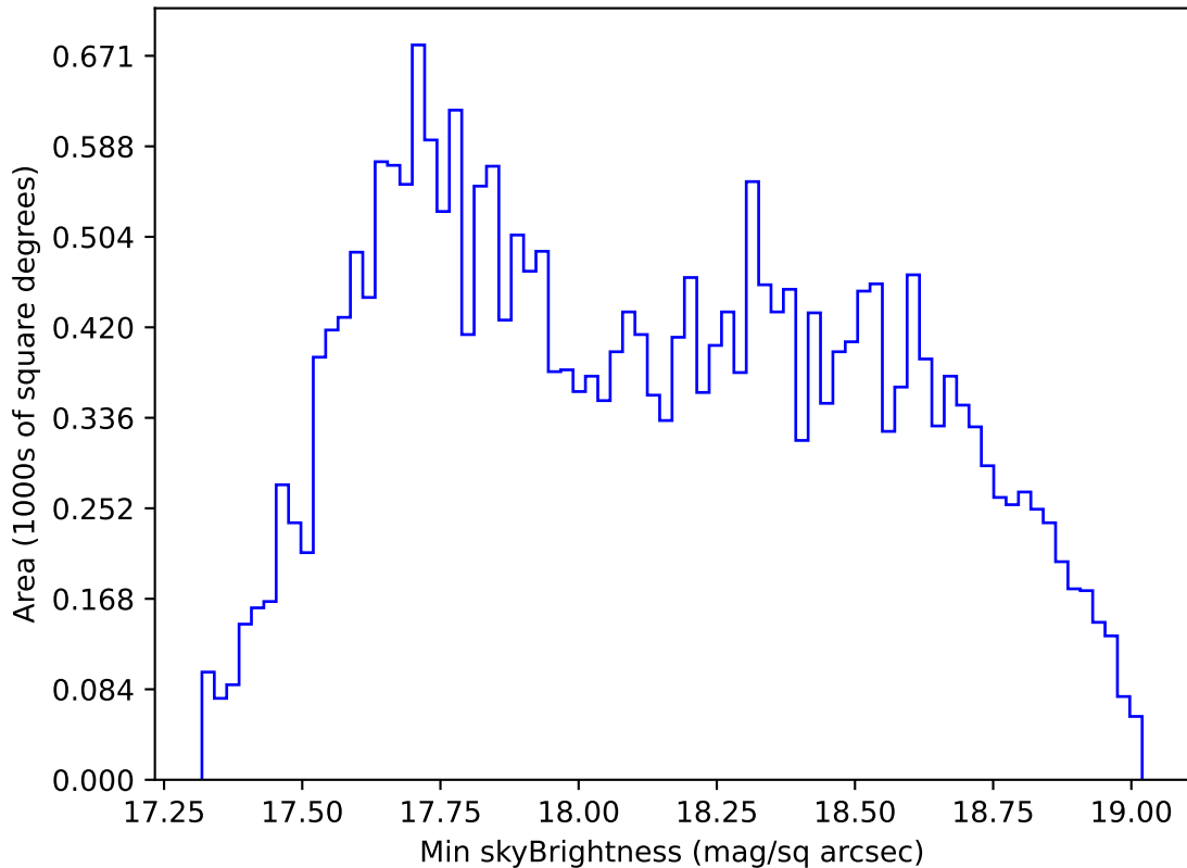
too_elab_heavy_r128_d3_griz_v3.4_10yrs All sky i band: Min skyBrightness
