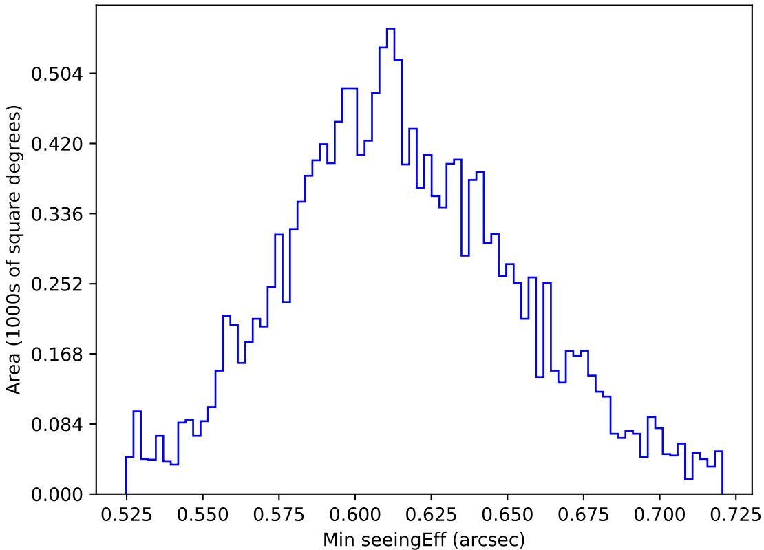
too_elab_heavy_r128_d3_griz_v3.4_10yrs WFD z band: Min seeingEff
