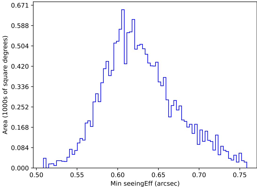
too_elab_heavy_r128_d3_griz_v3.4_10yrs WFD y band: Min seeingEff
