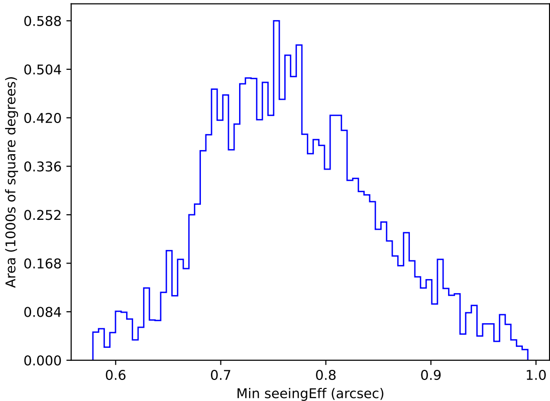
too_elab_heavy_r128_d3_griz_v3.4_10yrs WFD u band: Min seeingEff
