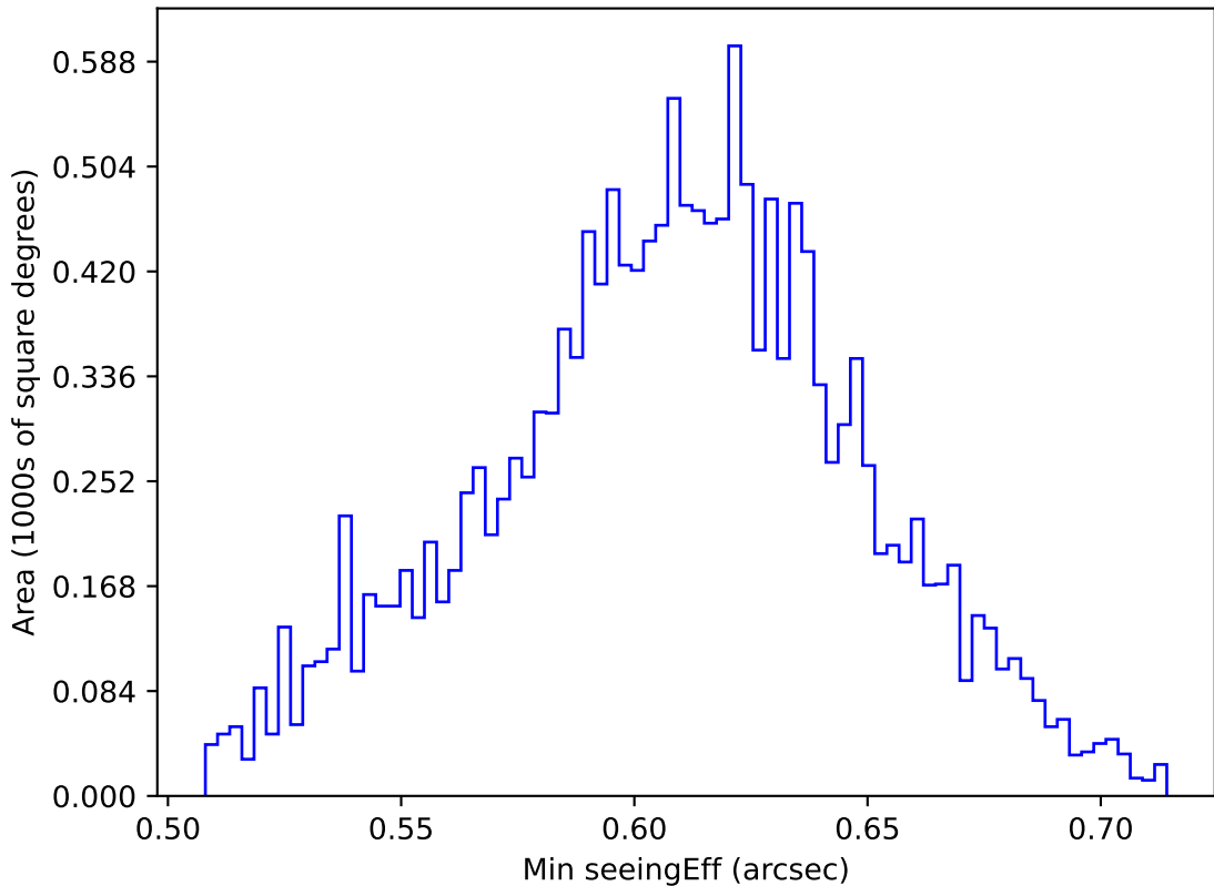
too_elab_heavy_r128_d3_griz_v3.4_10yrs WFD i band: Min seeingEff
