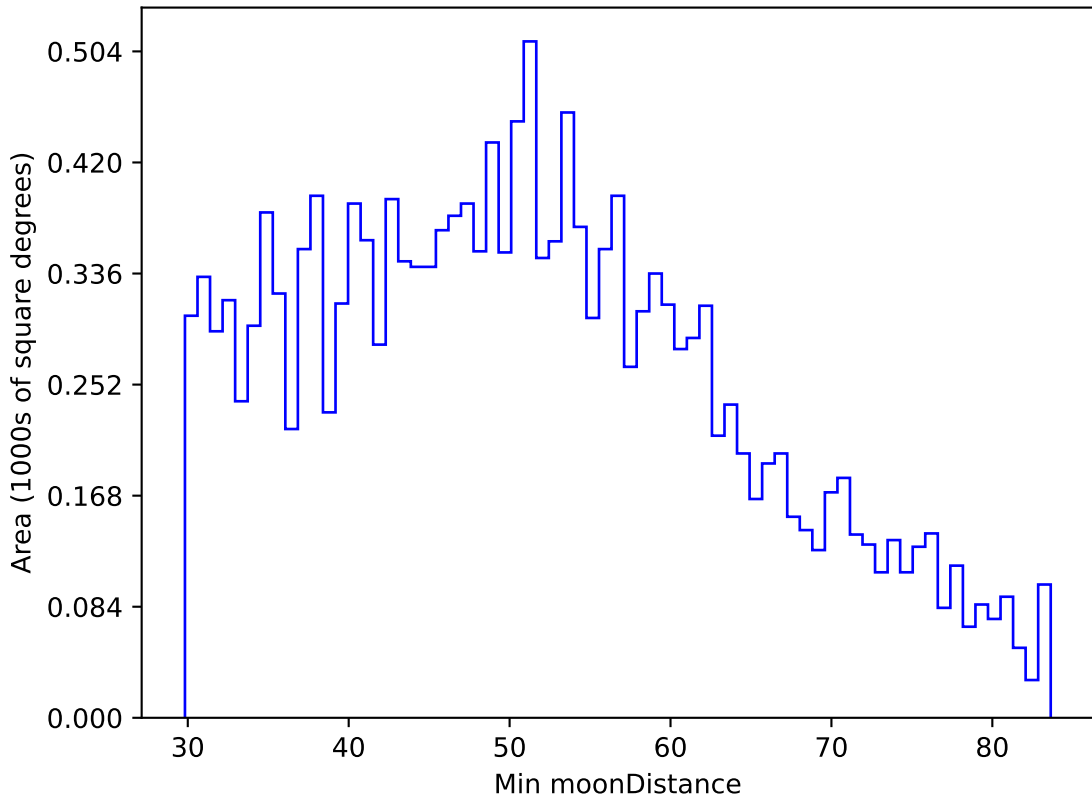
too_elab_heavy_r128_d3_griz_v3.4_10yrs WFD u band: Min moonDistance
