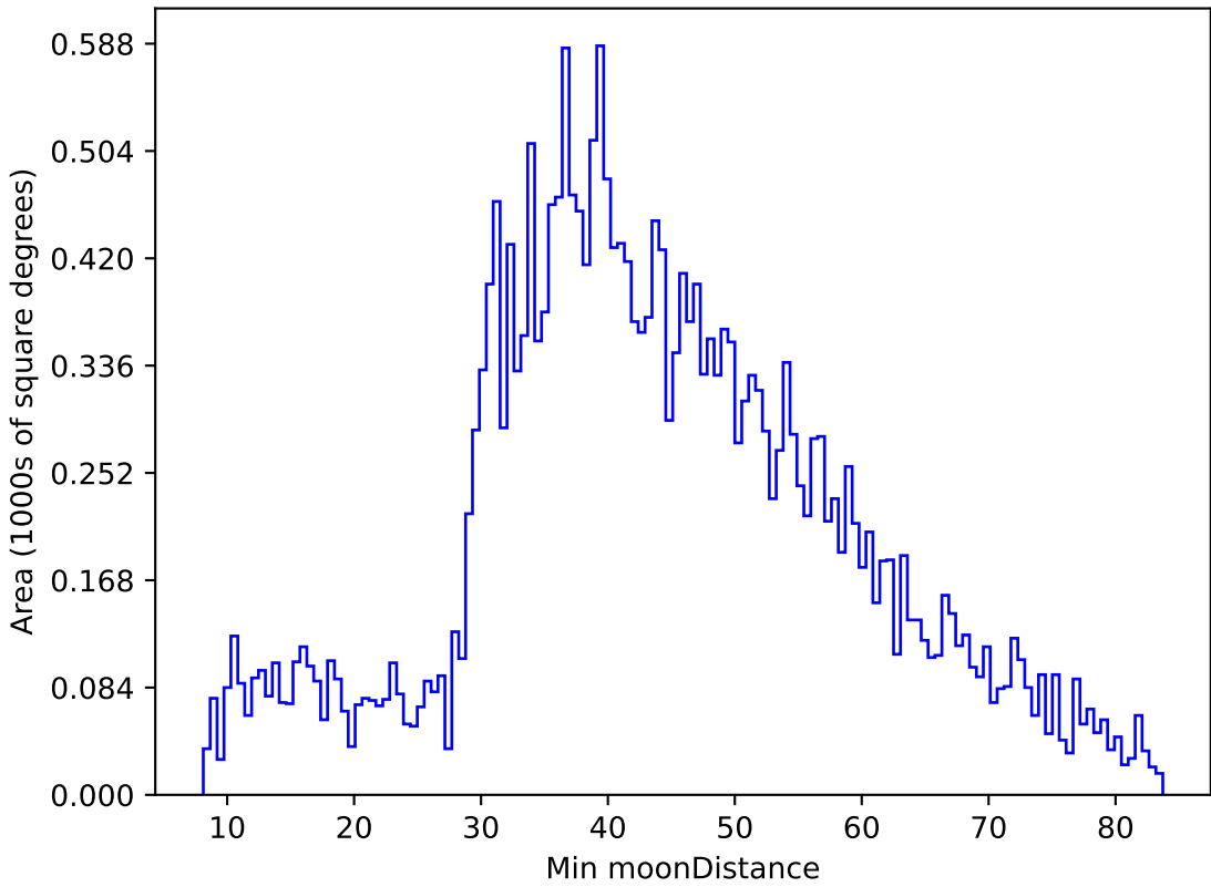
too_elab_heavy_r128_d3_griz_v3.4_10yrs All sky g band: Min moonDistance
