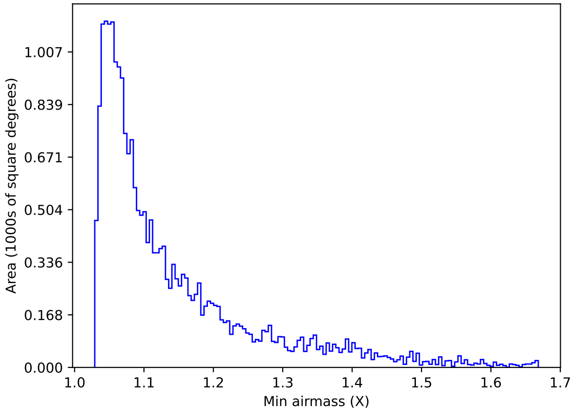
too_elab_heavy_r128_d3_griz_v3.4_10yrs Yr 1 u band: Min airmass
