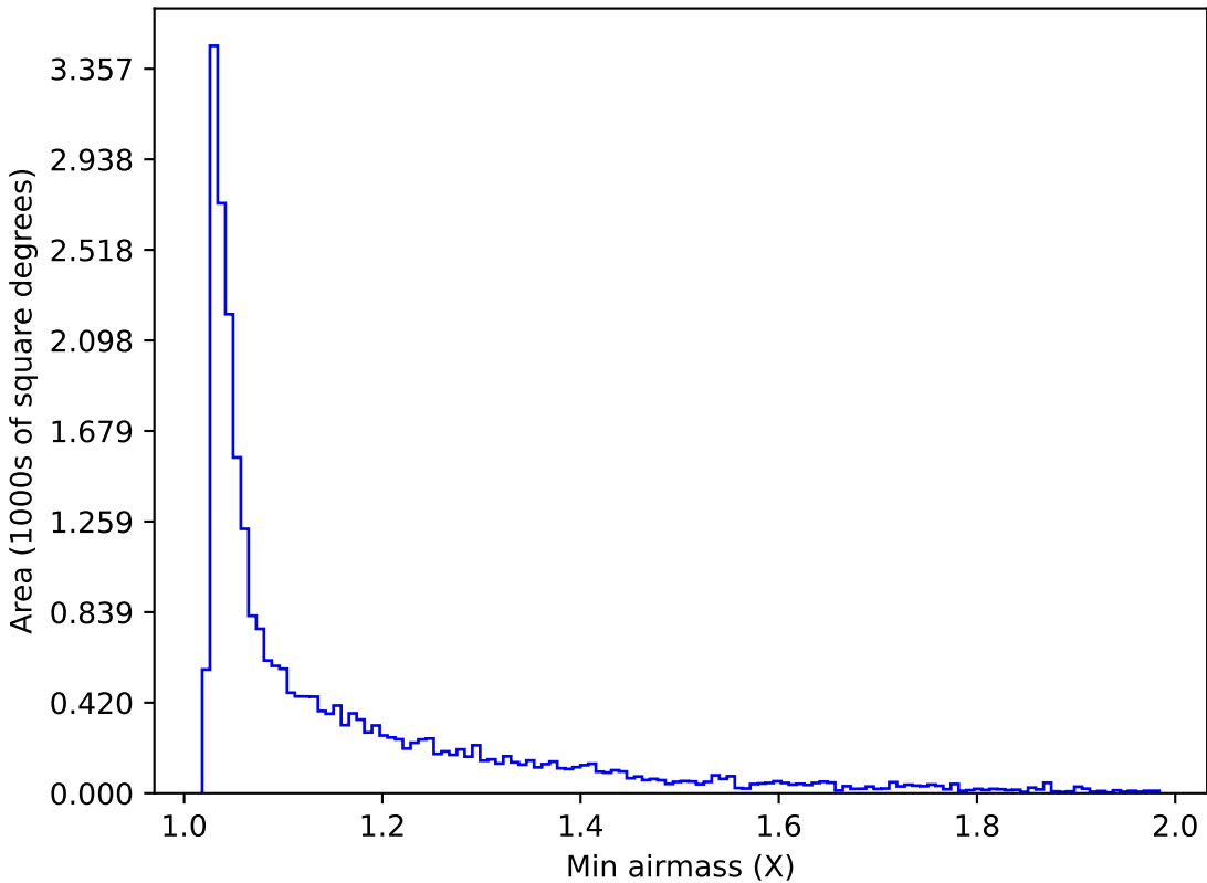
too_elab_heavy_r128_d3_griz_v3.4_10yrs Yr 1 i band: Min airmass
