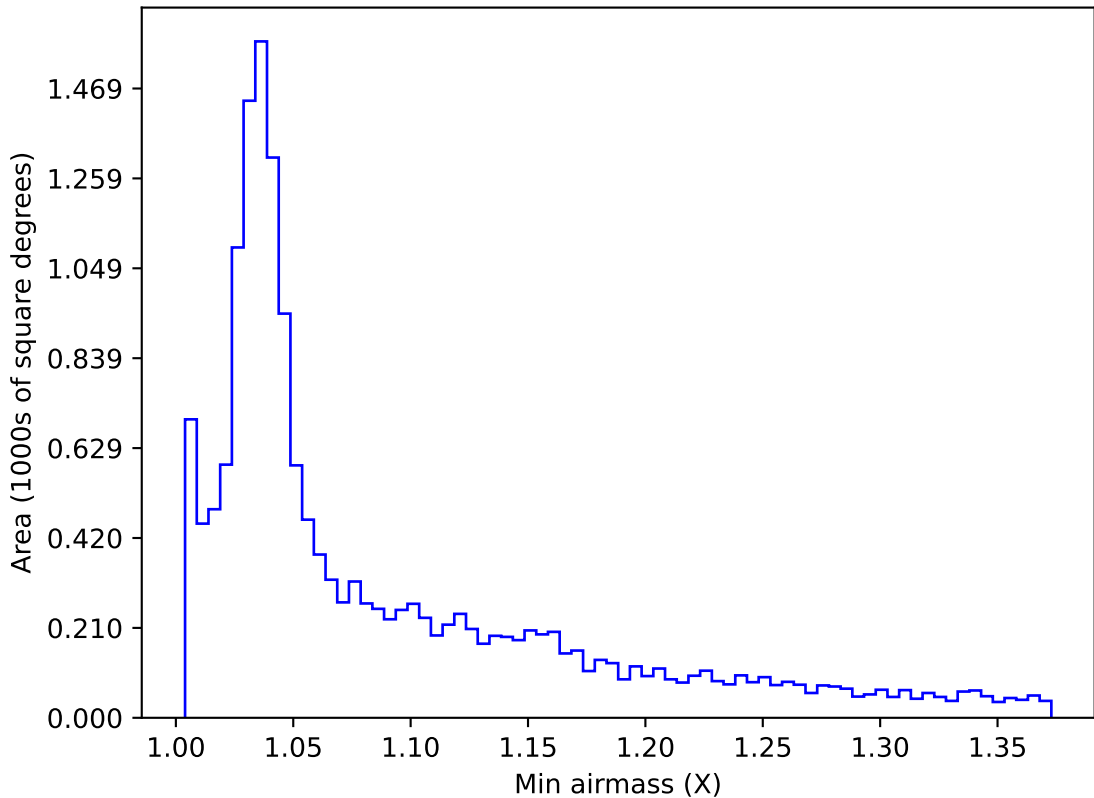
too_elab_heavy_r128_d3_griz_v3.4_10yrs WFD g band: Min airmass
