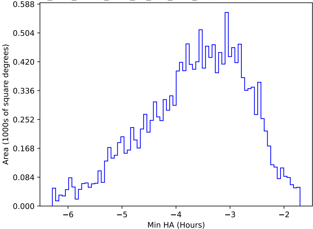
too_elab_heavy_r128_d3_griz_v3.4_10yrs WFD y band: Min HA
