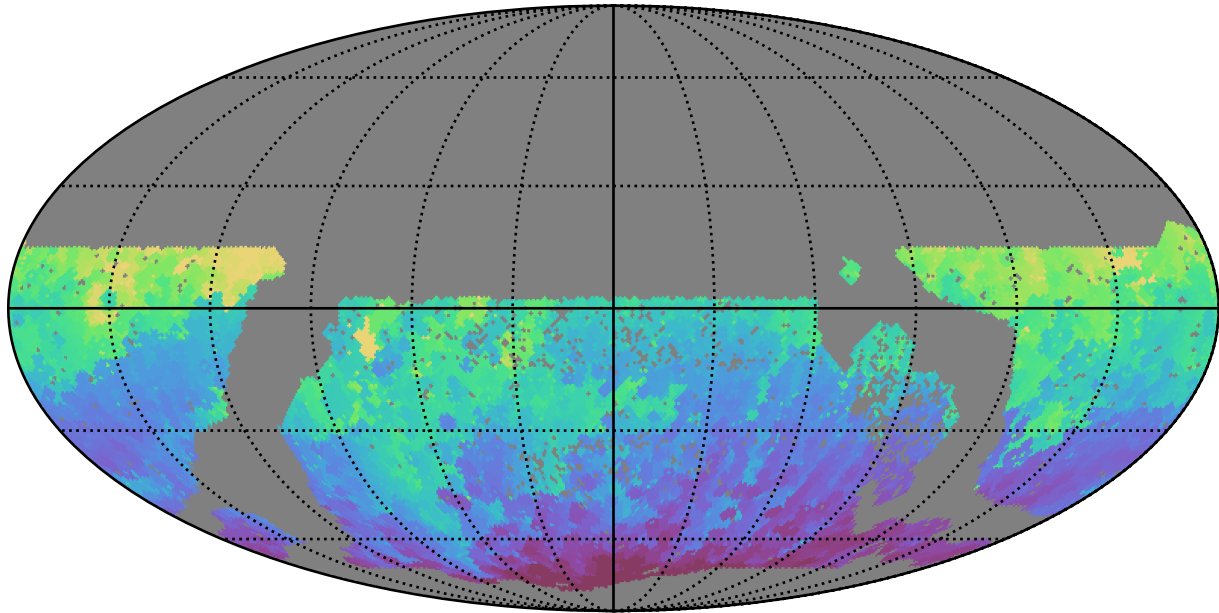
too_elab_heavy_r128_d3_griz_v3.4_10yrs WFD i band: Min HA
