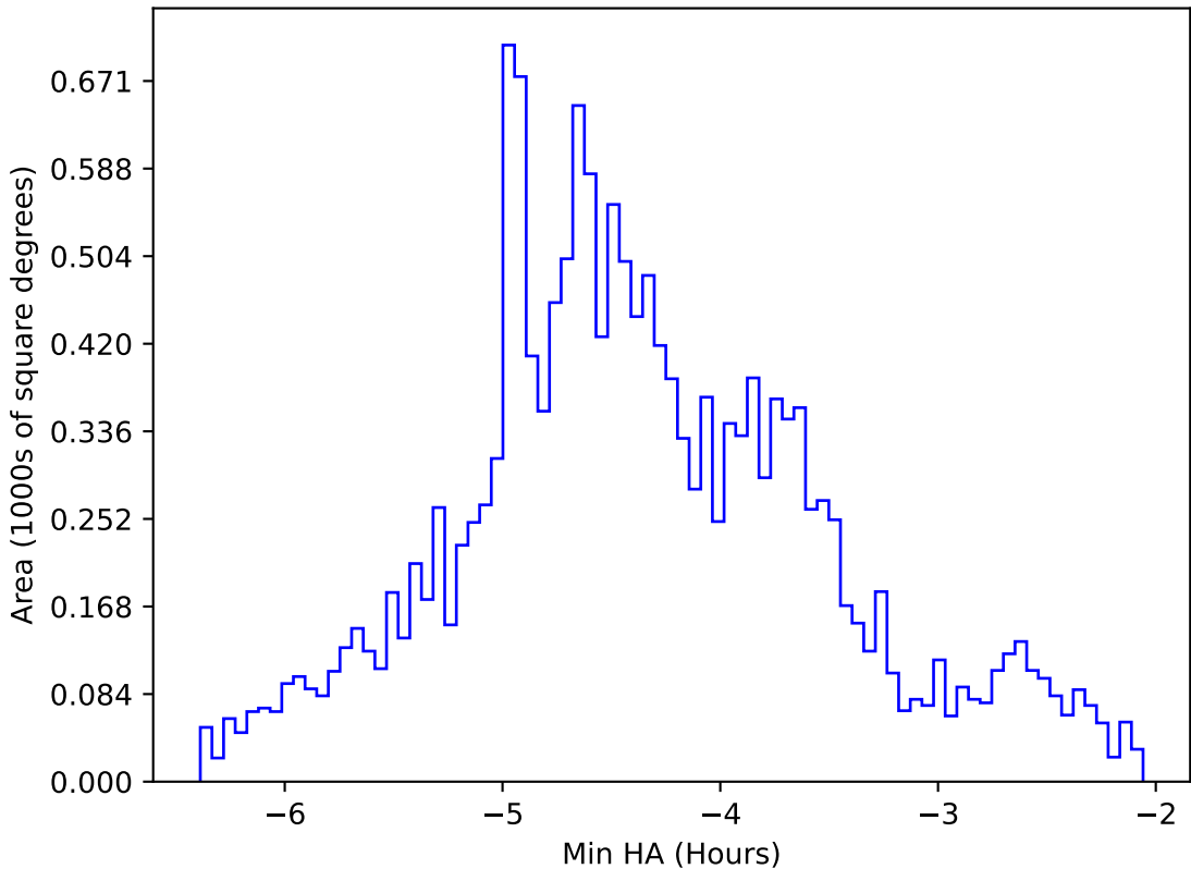
too_elab_heavy_r128_d3_griz_v3.4_10yrs WFD g band: Min HA
