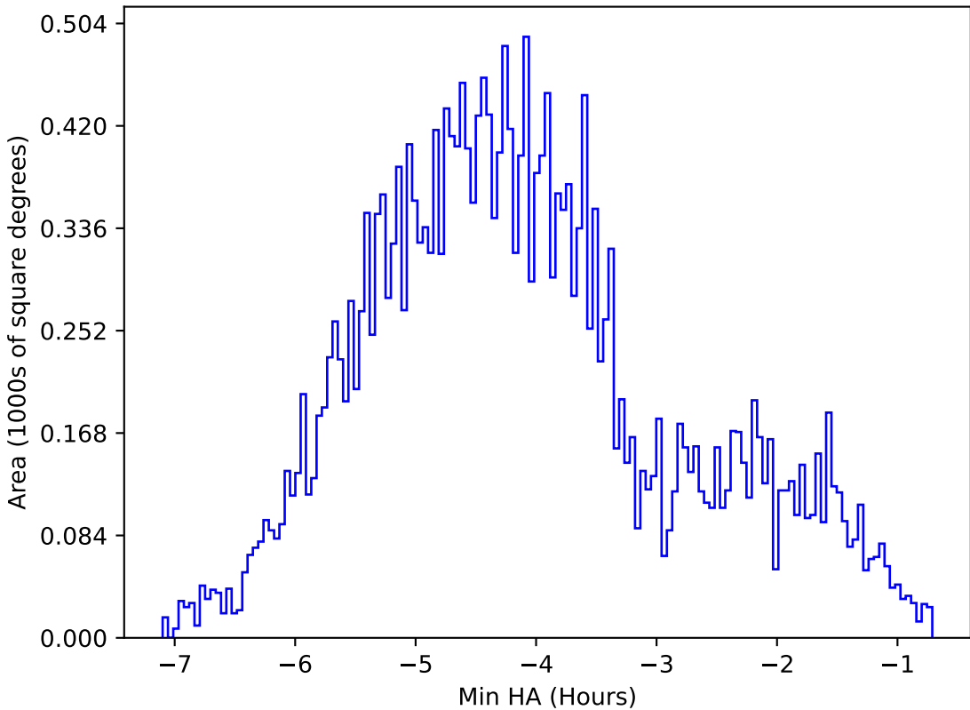
too_elab_heavy_r128_d3_griz_v3.4_10yrs All sky z band: Min HA
