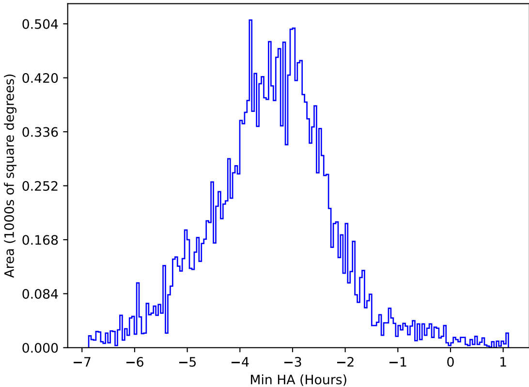
too_elab_heavy_r128_d3_griz_v3.4_10yrs All sky y band: Min HA
