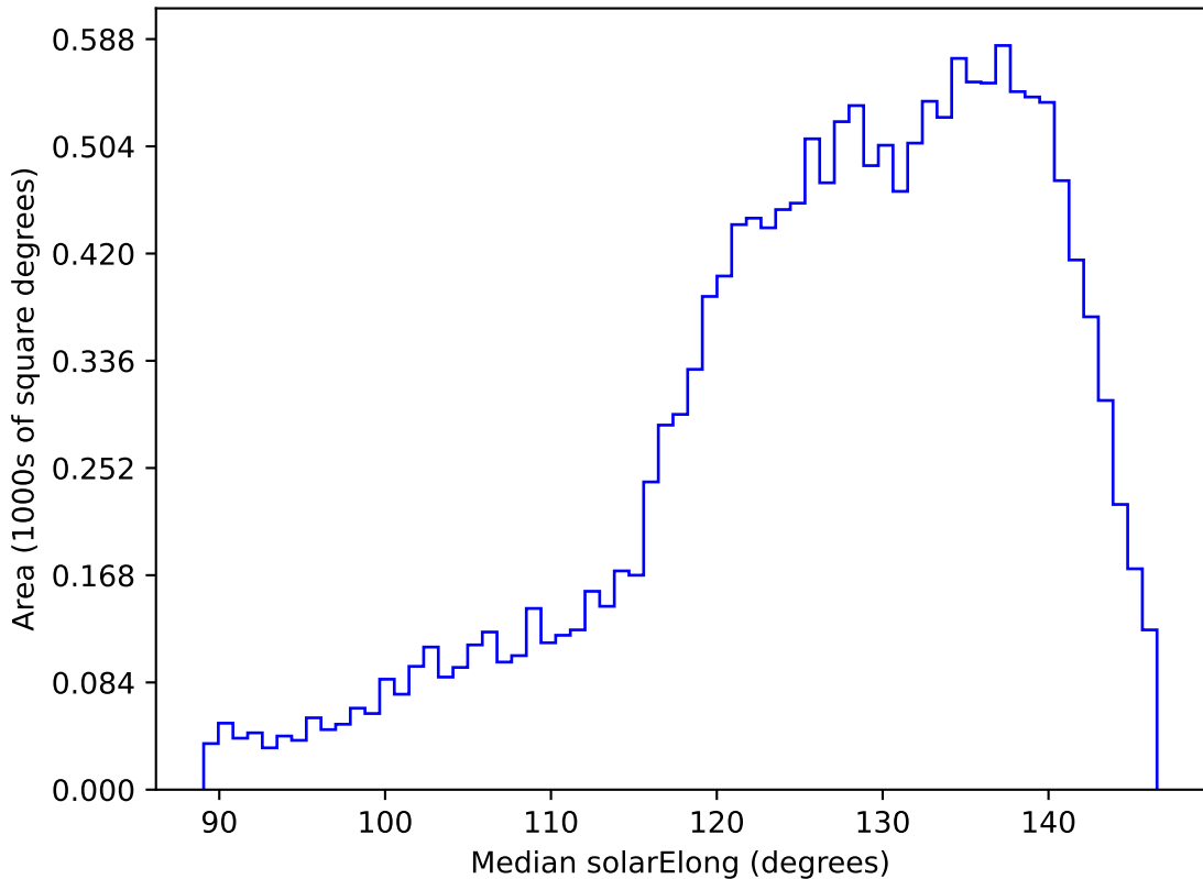
too_elab_heavy_r128_d3_griz_v3.4_10yrs WFD z band: Median solarElong
