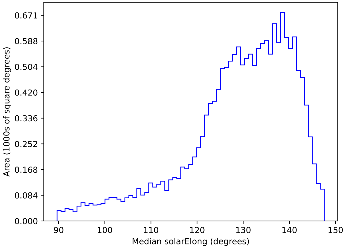
too_elab_heavy_r128_d3_griz_v3.4_10yrs WFD i band: Median solarElong
