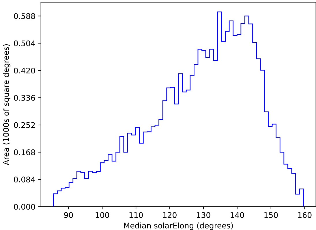
too_elab_heavy_r128_d3_griz_v3.4_10yrs WFD g band: Median solarElong
