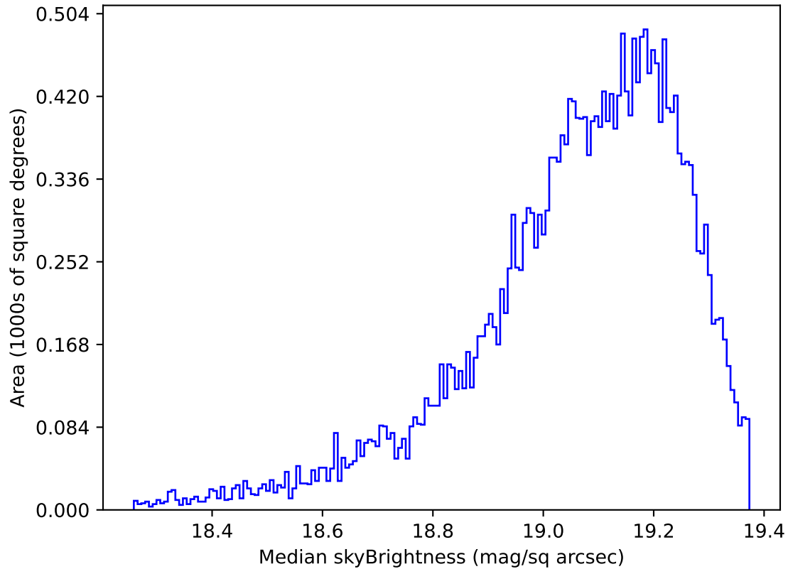
too_elab_heavy_r128_d3_griz_v3.4_10yrs Yr 1 z band: Median skyBrightness
