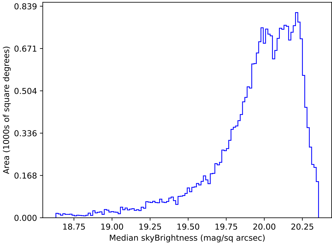
too_elab_heavy_r128_d3_griz_v3.4_10yrs Yr 1 i band: Median skyBrightness
