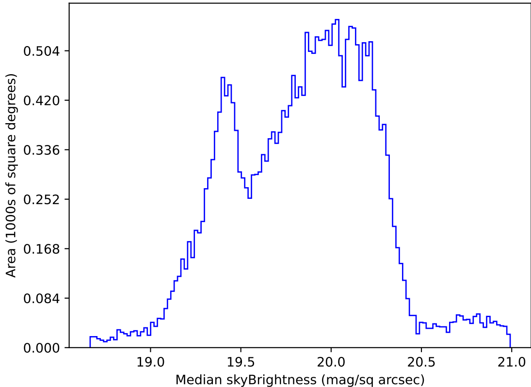
too_elab_heavy_r128_d3_griz_v3.4_10yrs Yr 1 all bands: Median skyBrightness
