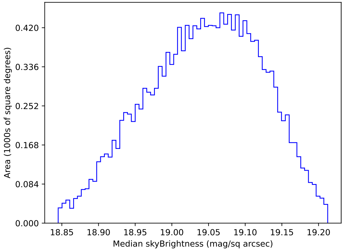
too_elab_heavy_r128_d3_griz_v3.4_10yrs WFD z band: Median skyBrightness
