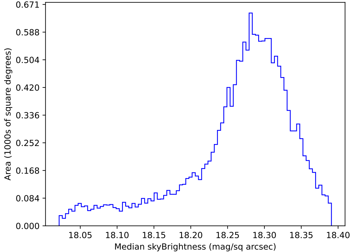
too_elab_heavy_r128_d3_griz_v3.4_10yrs WFD y band: Median skyBrightness
