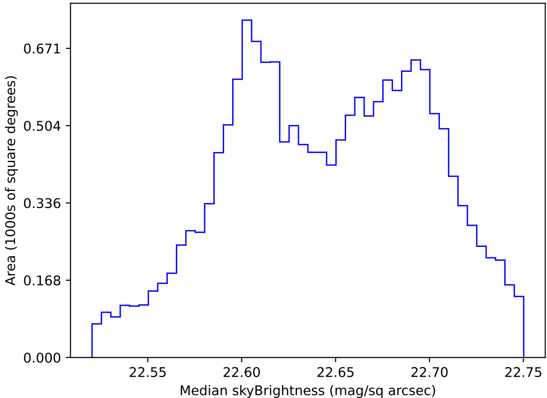
too_elab_heavy_r128_d3_griz_v3.4_10yrs WFD u band: Median skyBrightness
