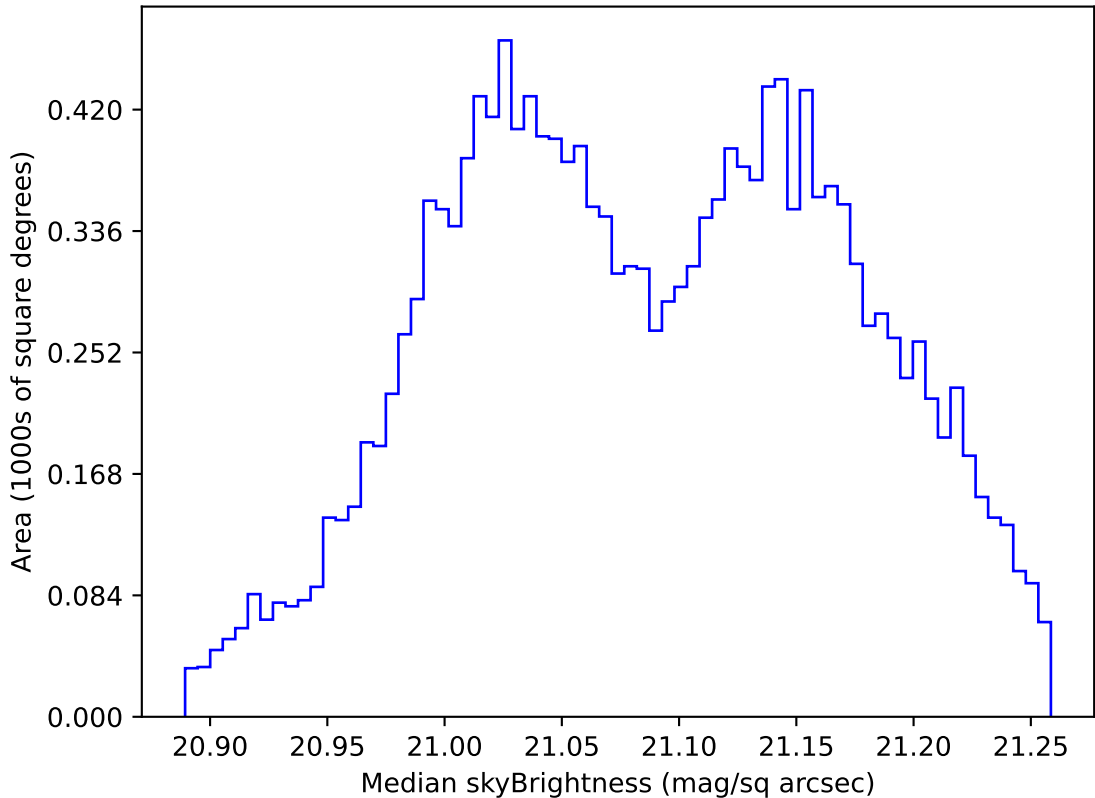
too_elab_heavy_r128_d3_griz_v3.4_10yrs WFD r band: Median skyBrightness
