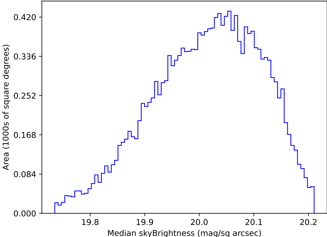
too_elab_heavy_r128_d3_griz_v3.4_10yrs WFD i band: Median skyBrightness
