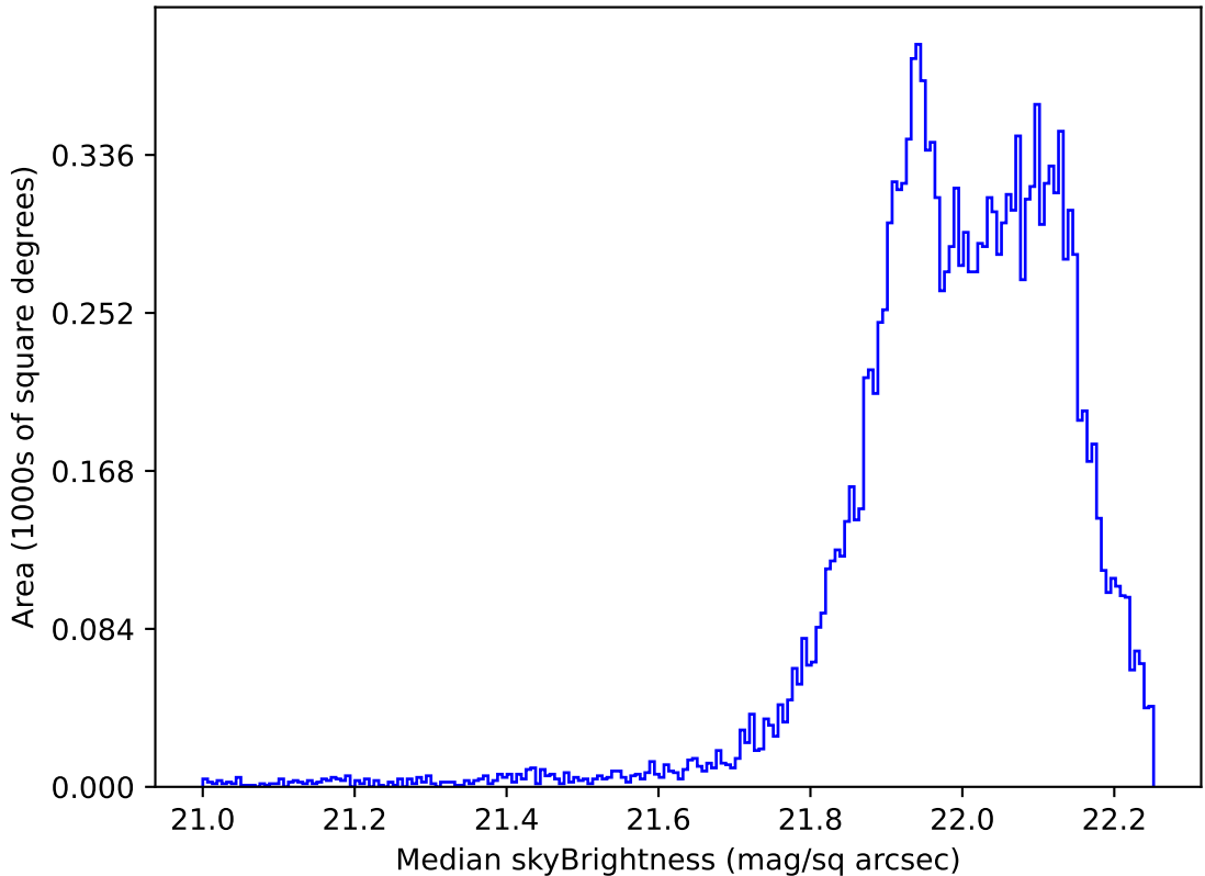
too_elab_heavy_r128_d3_griz_v3.4_10yrs WFD g band: Median skyBrightness
