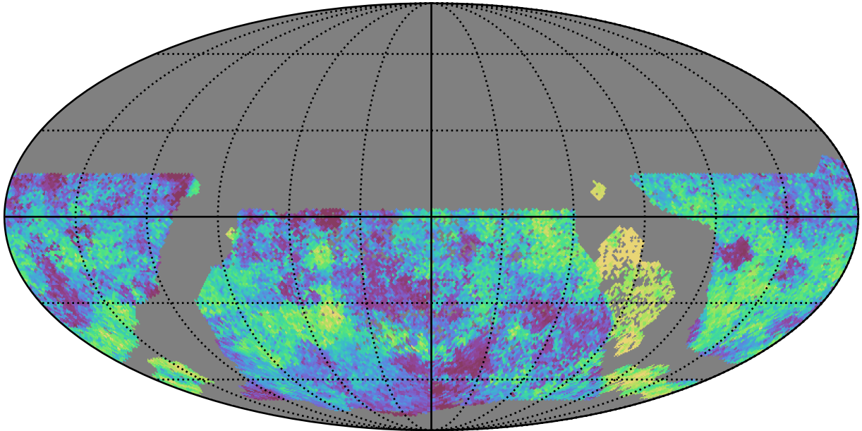
too_elab_heavy_r128_d3_griz_v3.4_10yrs WFD all bands: Median skyBrightness
