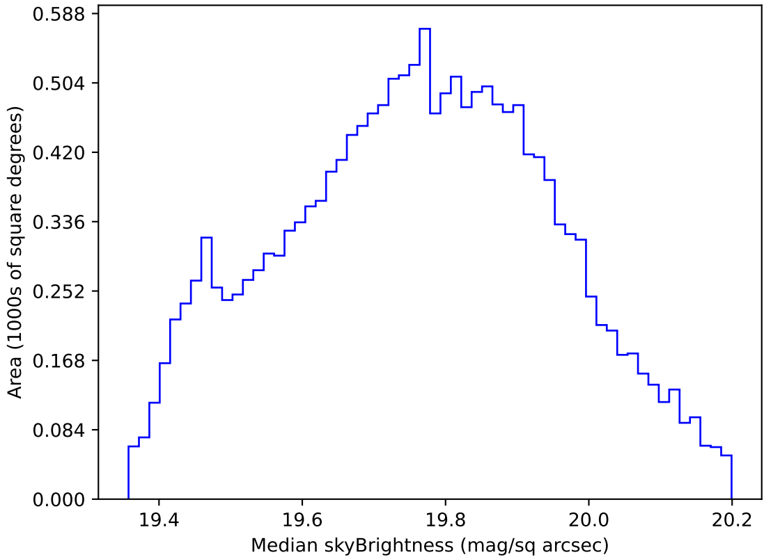
too_elab_heavy_r128_d3_griz_v3.4_10yrs WFD all bands: Median skyBrightness
