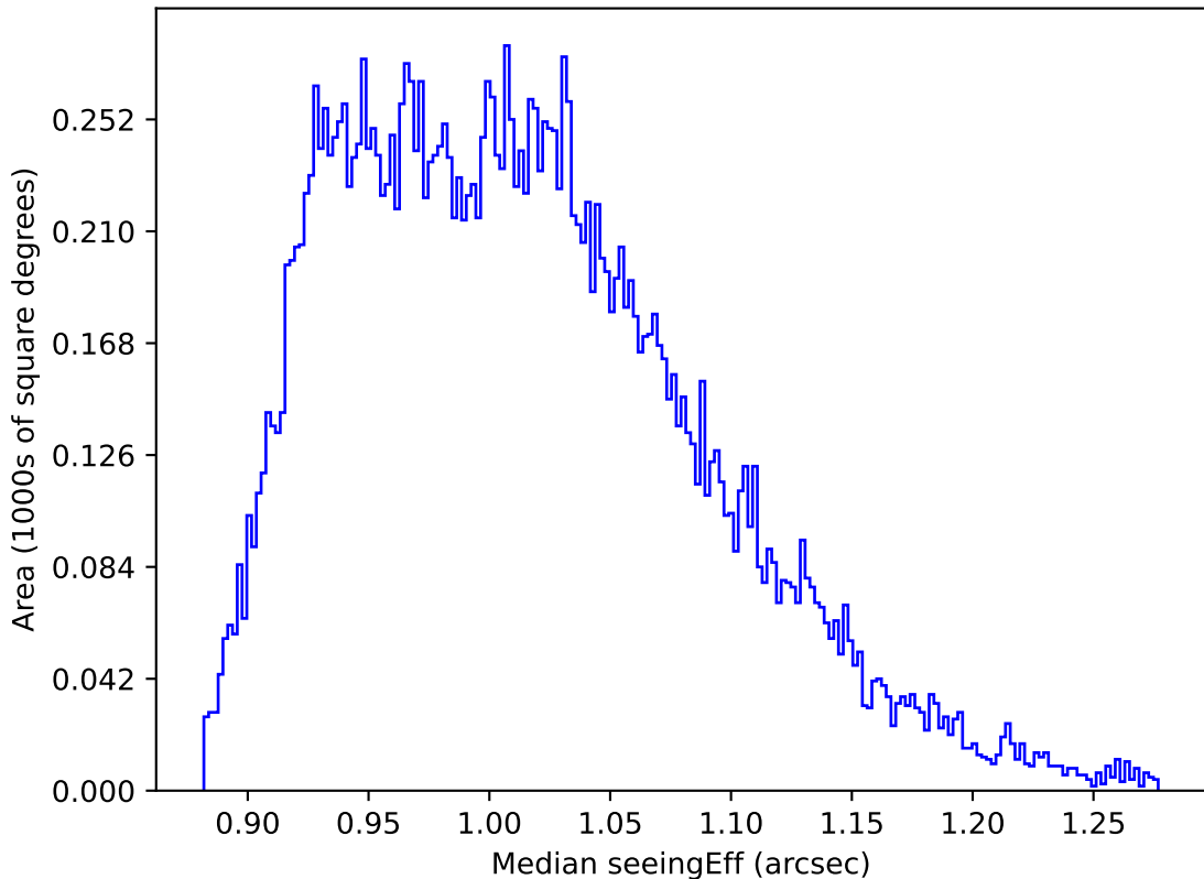
too_elab_heavy_r128_d3_griz_v3.4_10yrs All sky y band: Median seeingEff
