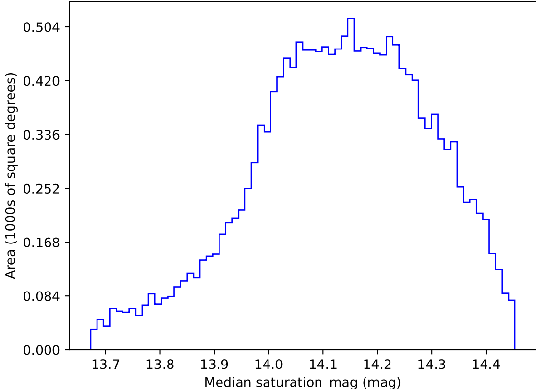
too_elab_heavy_r128_d3_griz_v3.4_10yrs WFD all bands: Median saturation_mag
