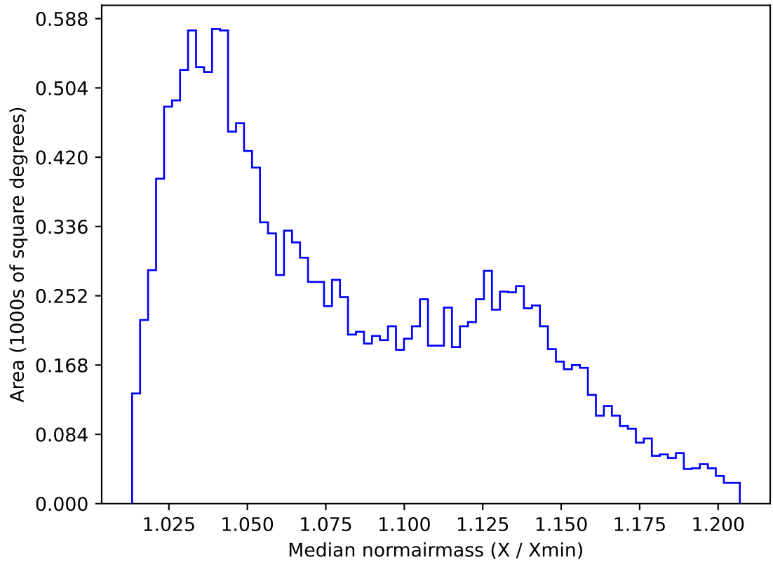
too_elab_heavy_r128_d3_griz_v3.4_10yrs WFD u band: Median normairmass
