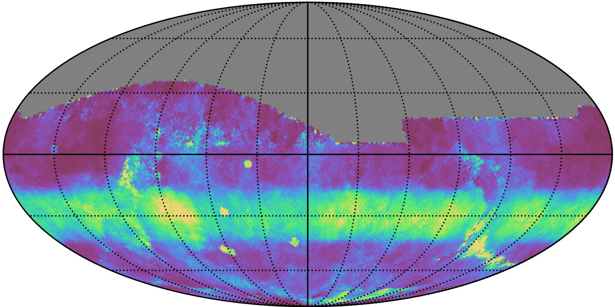
too_elab_heavy_r128_d3_griz_v3.4_10yrs All sky r band: Median normairmass
