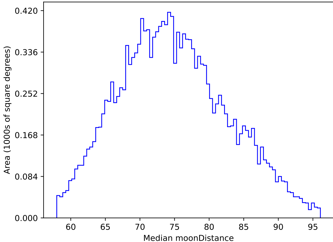
too_elab_heavy_r128_d3_griz_v3.4_10yrs WFD z band: Median moonDistance
