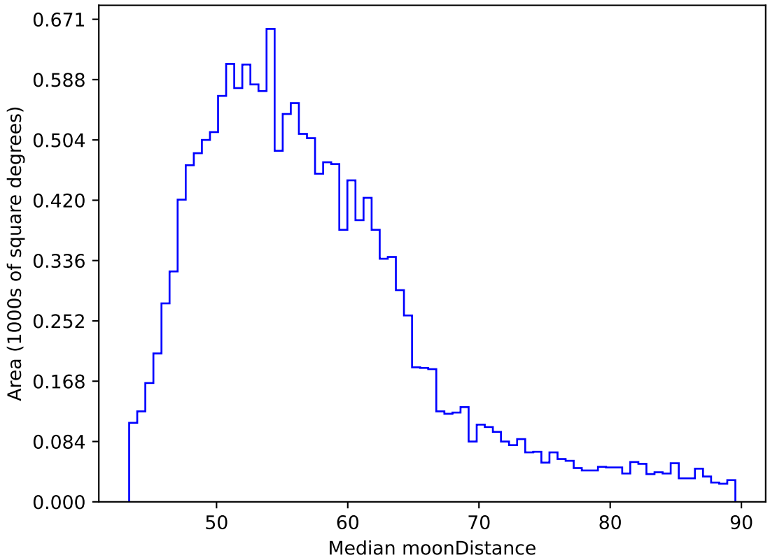
too_elab_heavy_r128_d3_griz_v3.4_10yrs WFD y band: Median moonDistance
