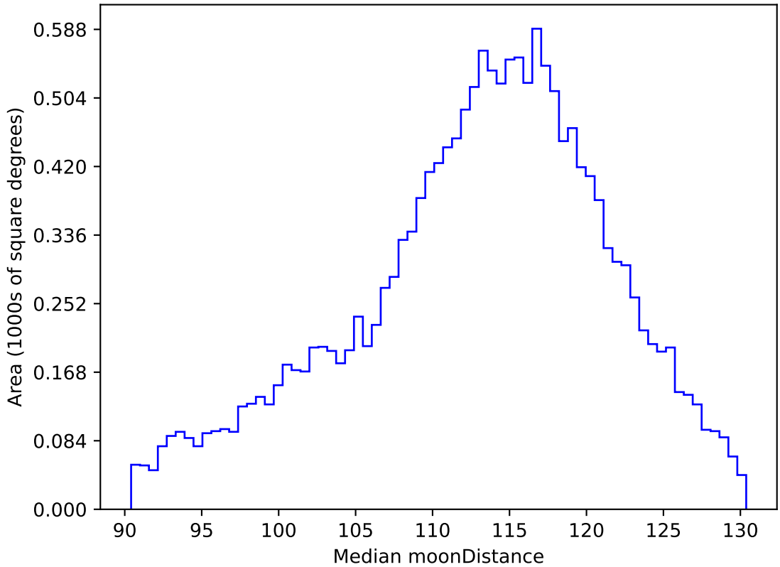
too_elab_heavy_r128_d3_griz_v3.4_10yrs WFD r band: Median moonDistance
