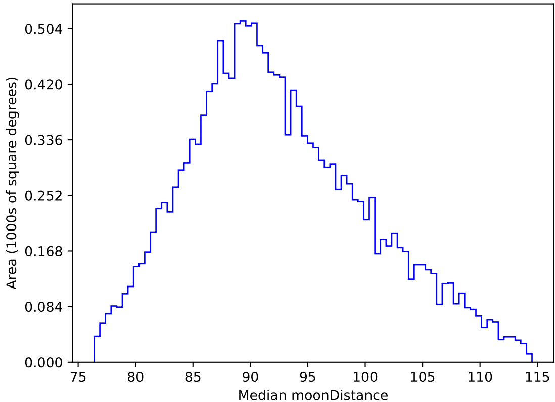
too_elab_heavy_r128_d3_griz_v3.4_10yrs WFD i band: Median moonDistance
