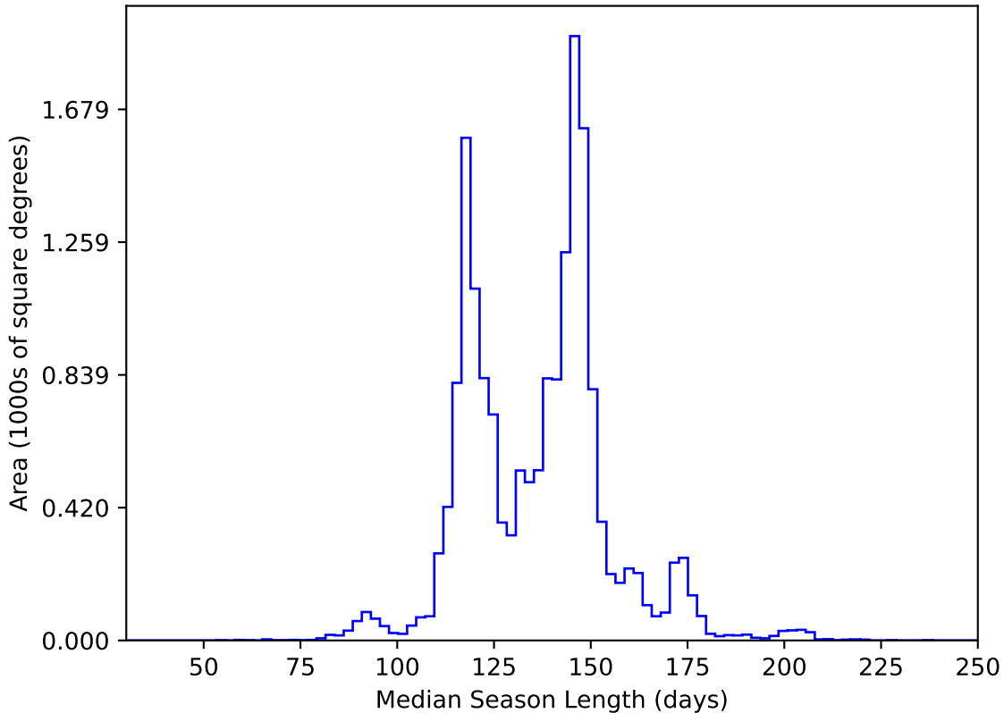
too_elab_heavy_r128_d3_griz_v3.4_10yrs WFD y band: Median Season Length
