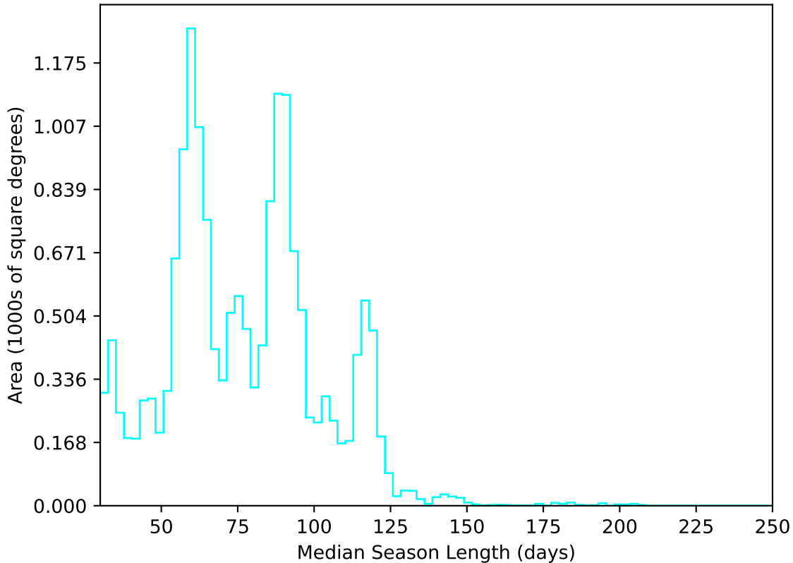
too_elab_heavy_r128_d3_griz_v3.4_10yrs WFD u band: Median Season Length
