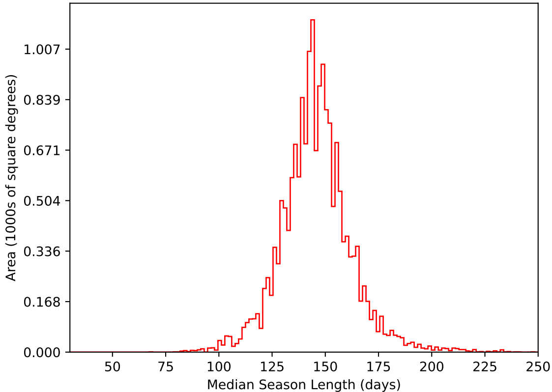
too_elab_heavy_r128_d3_griz_v3.4_10yrs WFD i band: Median Season Length
