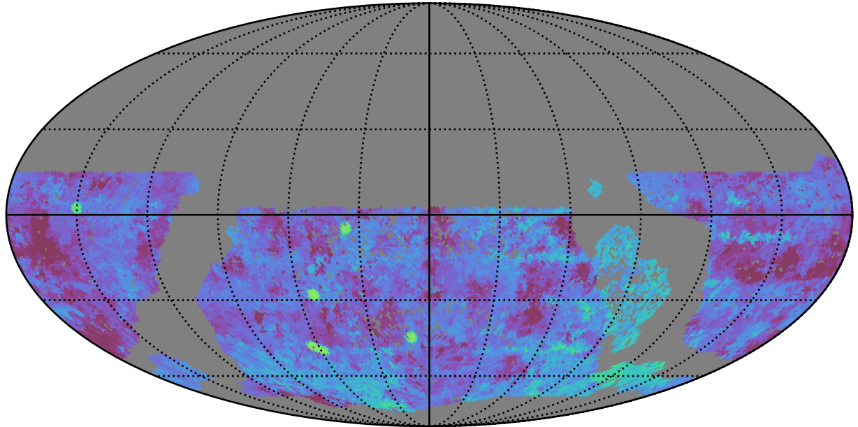
too_elab_heavy_r128_d3_griz_v3.4_10yrs WFD g band: Median Season Length
