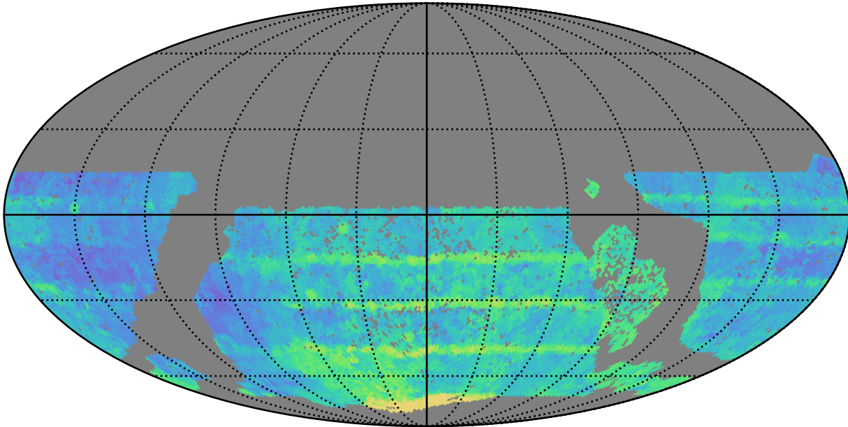
too_elab_heavy_r128_d3_griz_v3.4_10yrs WFD all bands: Median Season Length
