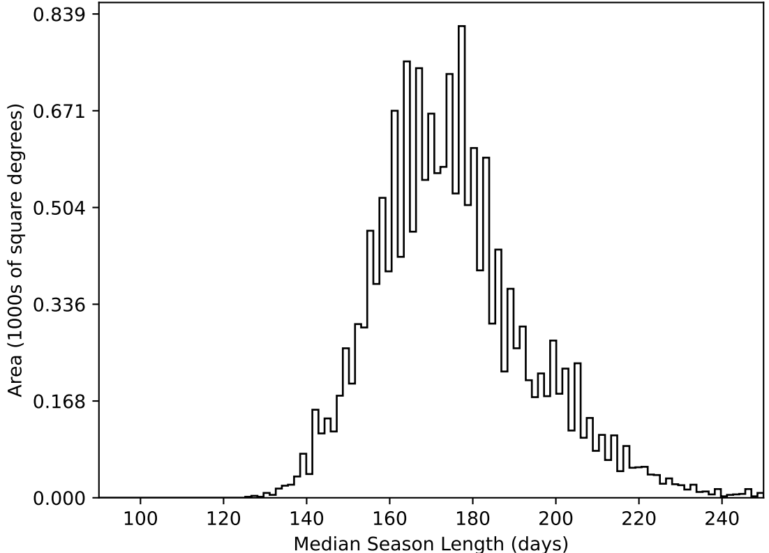
too_elab_heavy_r128_d3_griz_v3.4_10yrs WFD all bands: Median Season Length
