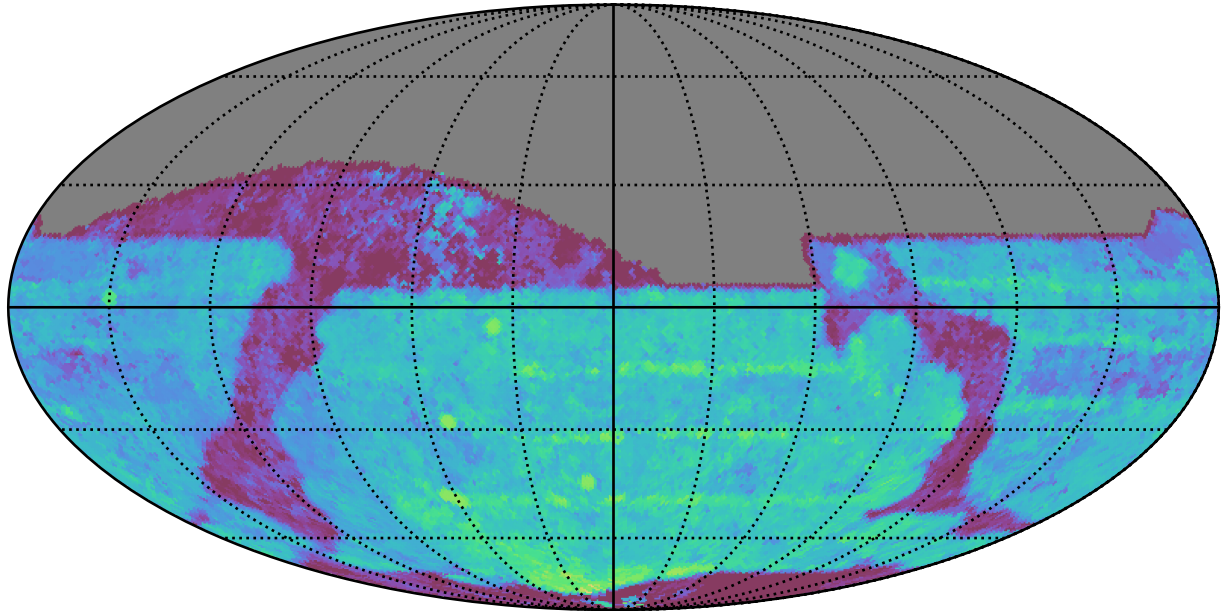
too_elab_heavy_r128_d3_griz_v3.4_10yrs All sky z band: Median Season Length
