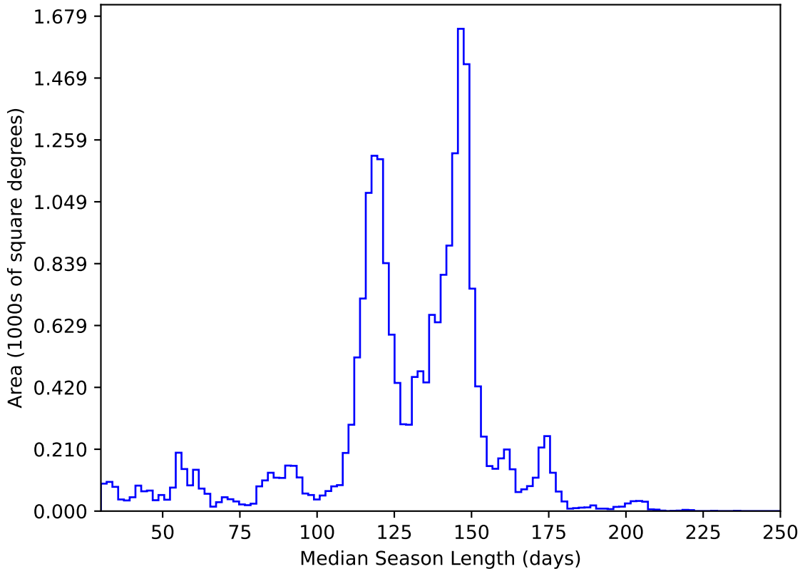
too_elab_heavy_r128_d3_griz_v3.4_10yrs All sky y band: Median Season Length
