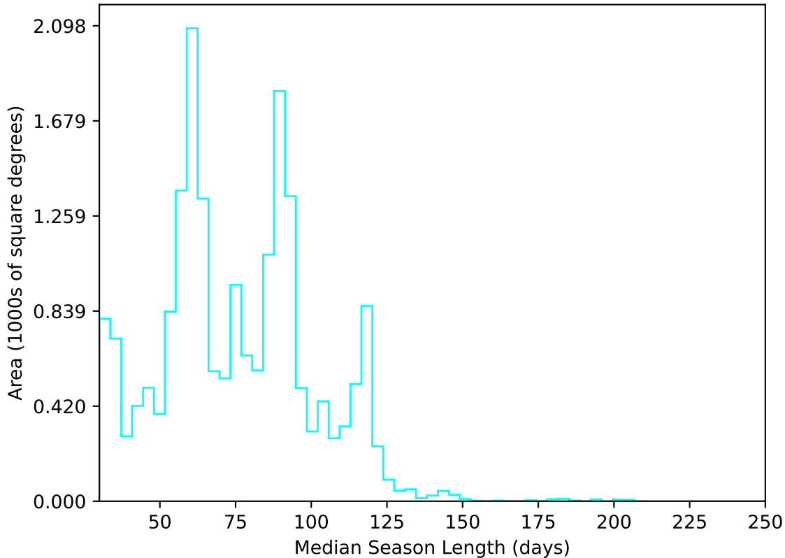
too_elab_heavy_r128_d3_griz_v3.4_10yrs All sky u band: Median Season Length
