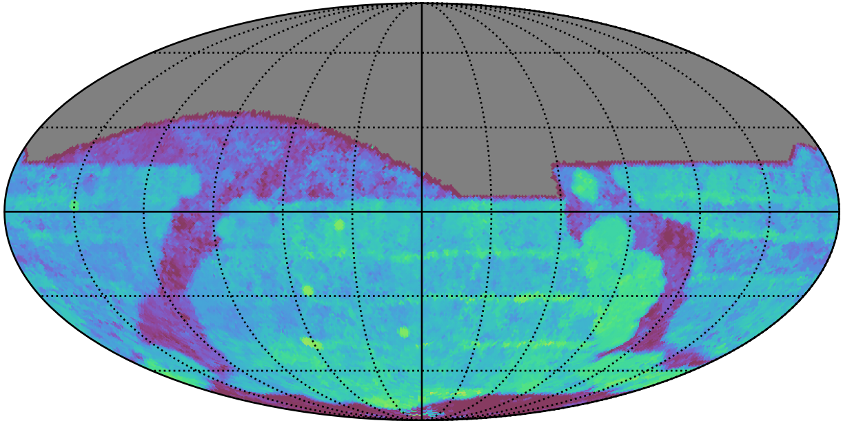
too_elab_heavy_r128_d3_griz_v3.4_10yrs All sky r band: Median Season Length
