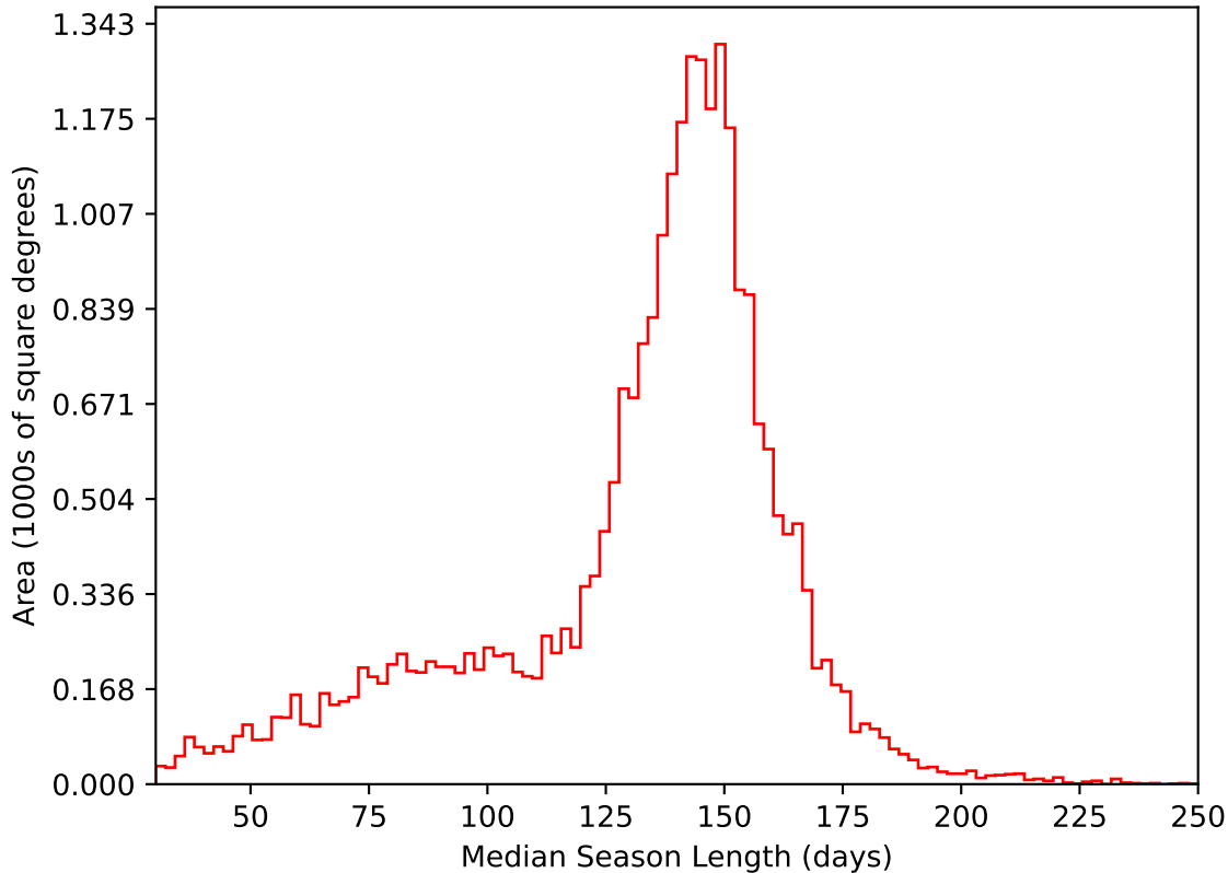
too_elab_heavy_r128_d3_griz_v3.4_10yrs All sky i band: Median Season Length
