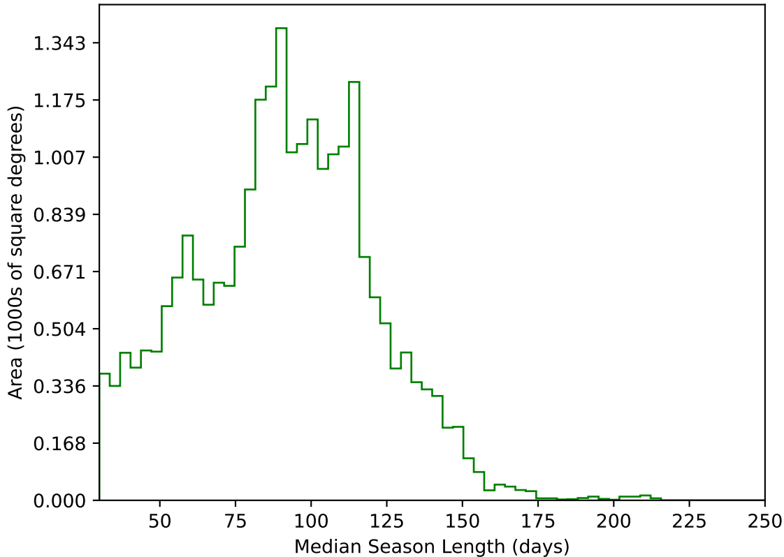
too_elab_heavy_r128_d3_griz_v3.4_10yrs All sky g band: Median Season Length
