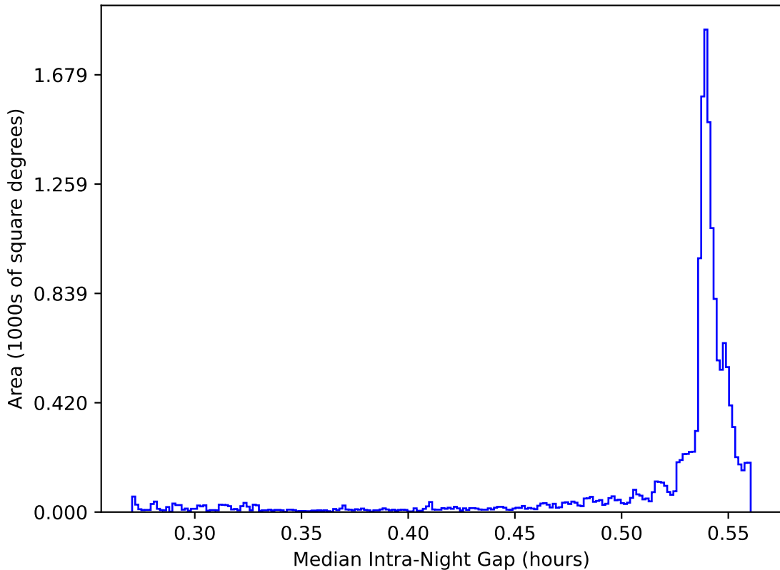
too_elab_heavy_r128_d3_griz_v3.4_10yrs WFD: Median Intra-Night Gap
